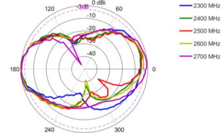
Elevation: 2300 – 2700 MHz
